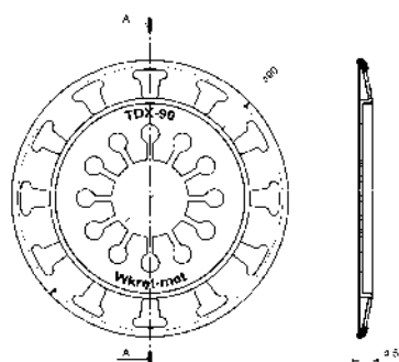
TDX-P-90/TDX-90
