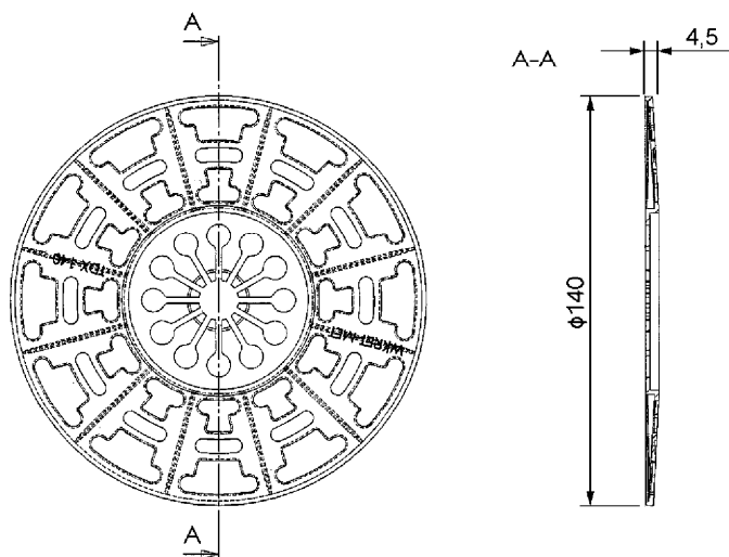
TDX-P-140/TDX-140
